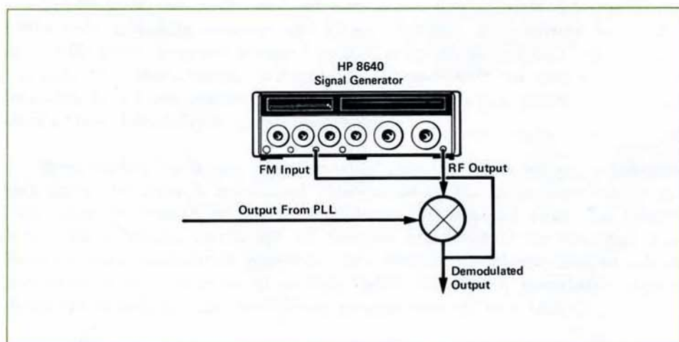
Figure 16. Setup using an 8640 Signal Generator to replace 8660 #2.
