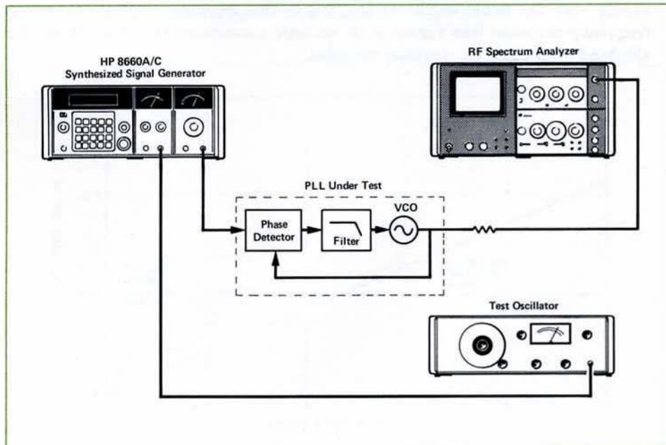
Figure 8. PLL Analysis Setup Using An RF Spectrum Analyzer.
