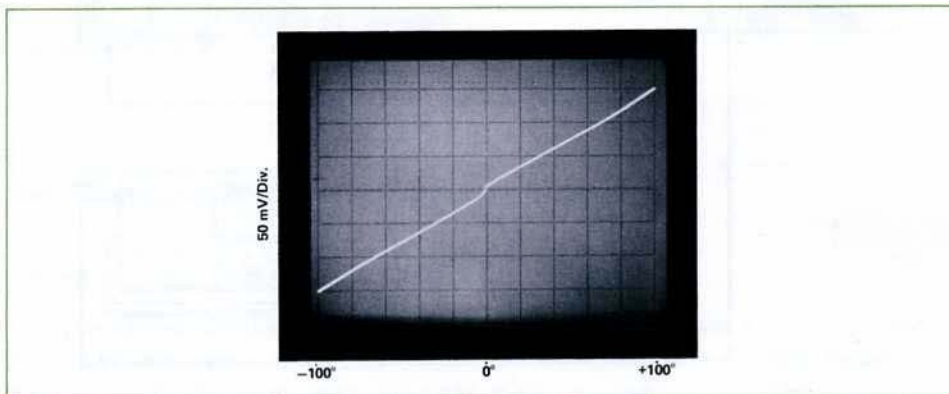
Figure 15. Phase-Frequency Detector Phase/Amplitude Characteristic Obtained Using the Test Setup Shown in Figure 12.
