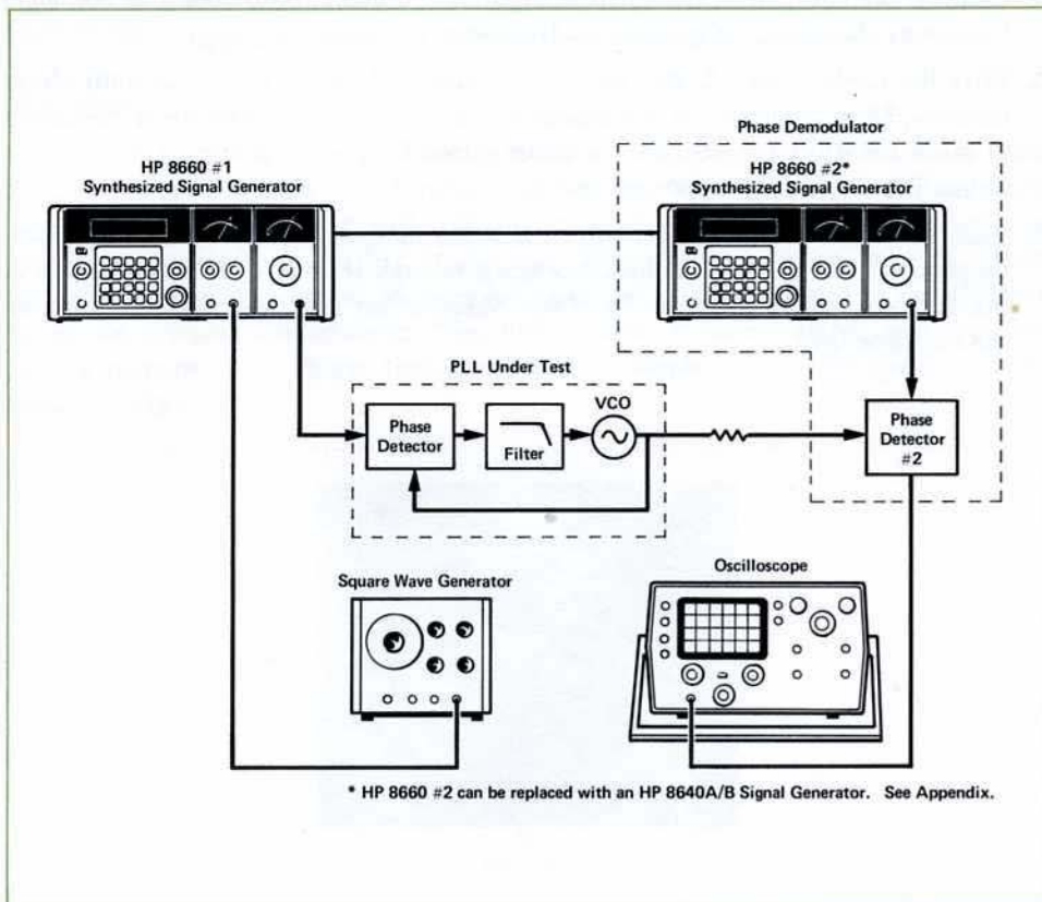
Figure 10. PLL Transient Analysis Test Setup.
