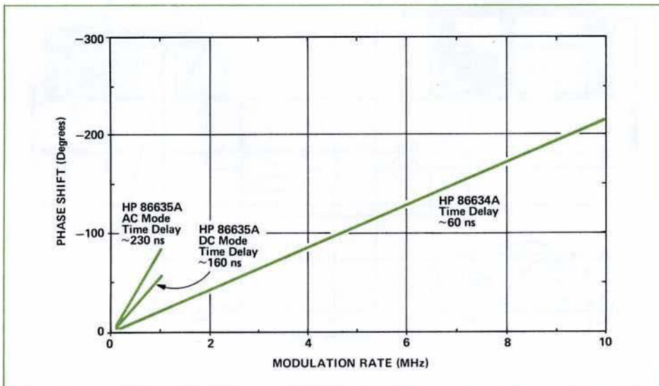
Figure 6. Typical Phase Shift of 8660 \phi M Measured from Modulation Section Input to RF Section Output.
