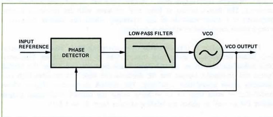
Figure 1. Simple PLL Block Diagram.
