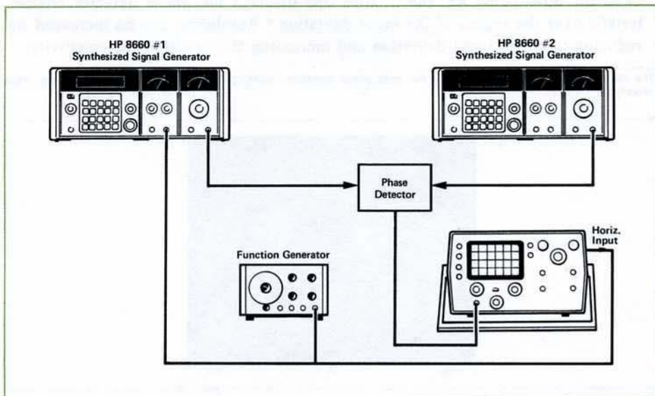
Figure 13. Phase Detector Characterization Test Setup.
