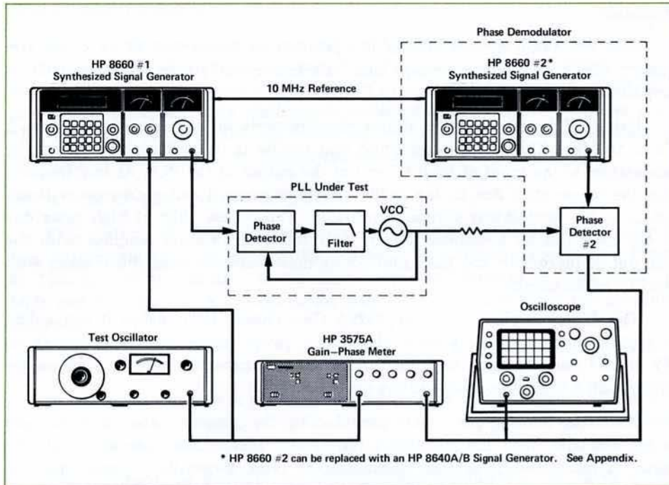
Figure 5. PLL Analysis Setup Using a Gain-Phase Meter.
