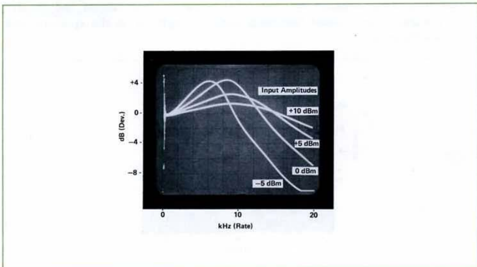
Figure 4. Variation of Frequency Response With Input Amplitude Obtained Using Test Setup Shown in Figure 2.
