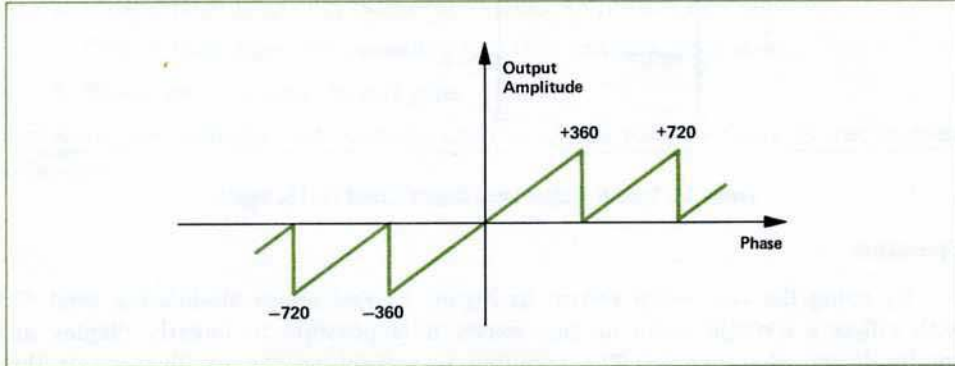
Figure 12. Typical Phase-Frequency Detector Phase/Amplitude Characteristic.
